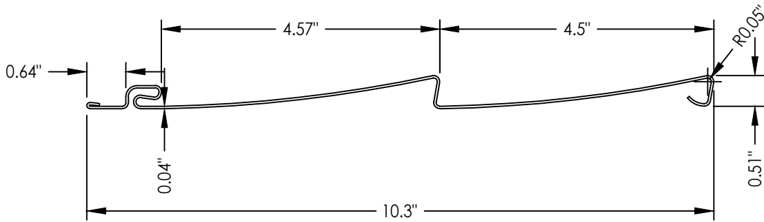
"Aurora II" D4.5 CLAPBOARD
