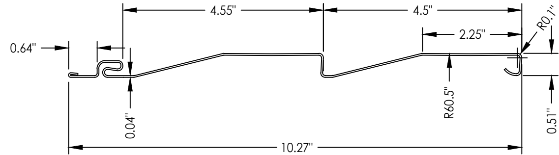
"Aurora II" D4.5 DUTCH LAP
