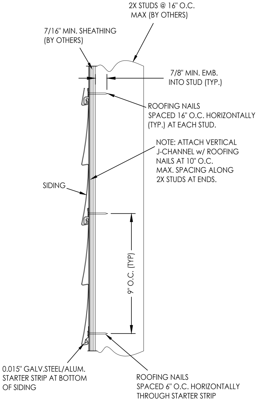
VERTICAL CROSS SECTION 2x stud construction w/ sheathing
